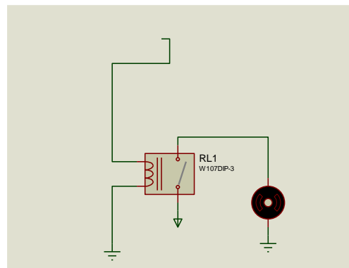
Figure 6 : Fire Pump Circuit
