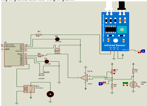
Figure 4 : Input & Outputs
