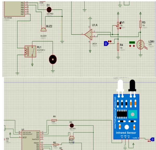
Figure 5 : Alarm Circuit (LDR & INFRARED)
